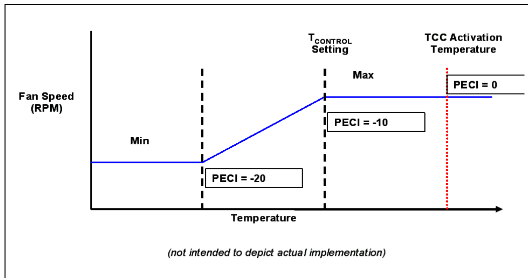
Figure 18. Conceptual Fan Control Diagram on PEFI-Based Platforms
