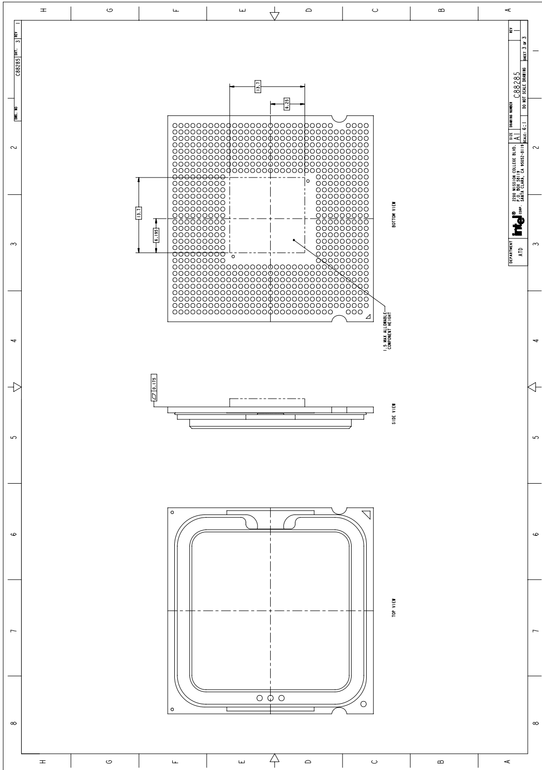
Figure 9. Processor Package Drawing Sheet 3 of 3
